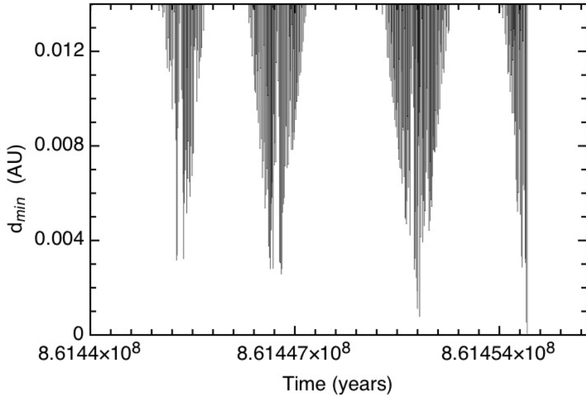
Fig. 10.— The minimal distance of approach during a series of close encounters between Mercury and Venus as a function of time. The collision takes place at t \sim 861.455 Myr, when d_{min} = 5.5561 \times 10^{-5} AU < r_{venus} + r_{mercury} = 5.6762 \times 10^{-5} AU.
